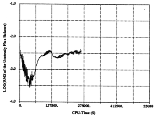
Fig. 10 Correction storage method with freezing Jacobian matrix.
