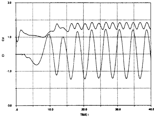
Fig. 5 Time evolution of the lift and the drag coefficients for Re_\infty=1000
